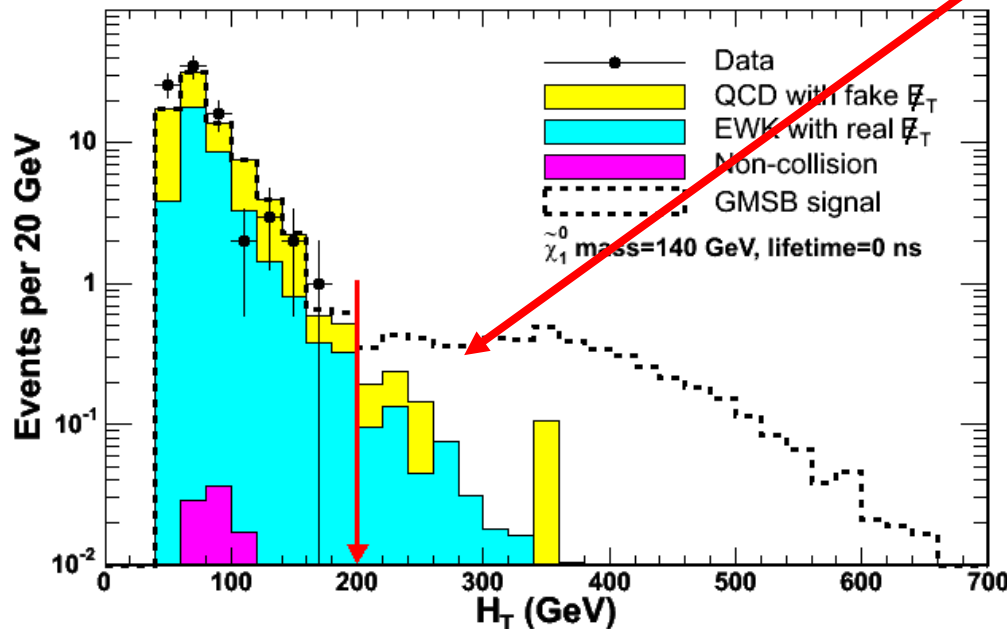
CDF Run II Preliminary, 2.6 fb -1
